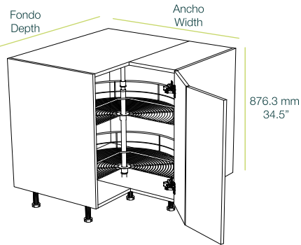
Base blind corner cabinet 1 puerta - BBC45
