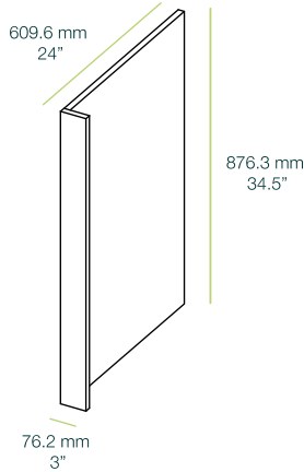
Dishwasher end panel - Tablero 18 mm / 3/4" board
