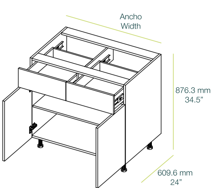
2 puertas - 2 cajones 2 doors - 2 drawers
